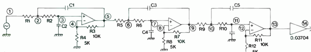
Seventh-order active elliptical filter used in Modulation Sciences MTS filter.
