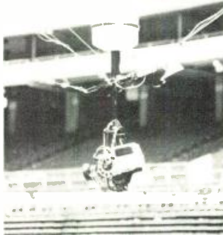
Suspended from four steel cables attached to pulley, Skyworks' Skycam "flies" over a baseball stadium with camera mounted to a gyro-stabilized base.
