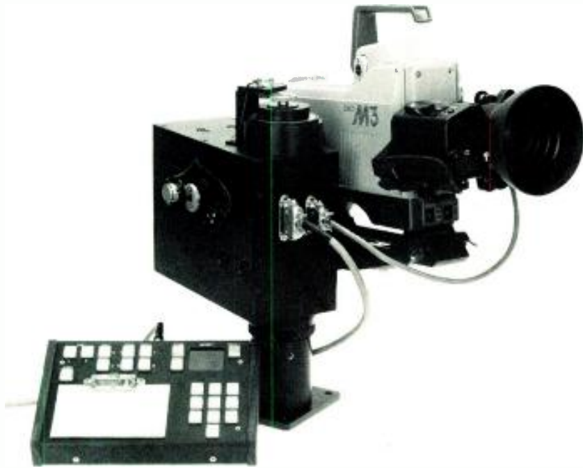
TSM Inc. has designed a streamlined, four-camera version of this HS 100P microprocessor-controlled remote system for broadcast use.
