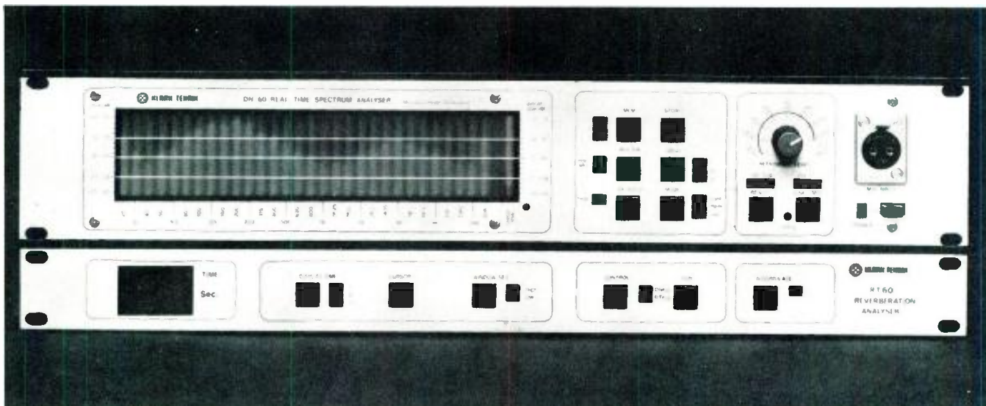
This real-time spectrum analyzer from Klark Teknik, with LED bargraph display, can be programmed for automatic tests.
